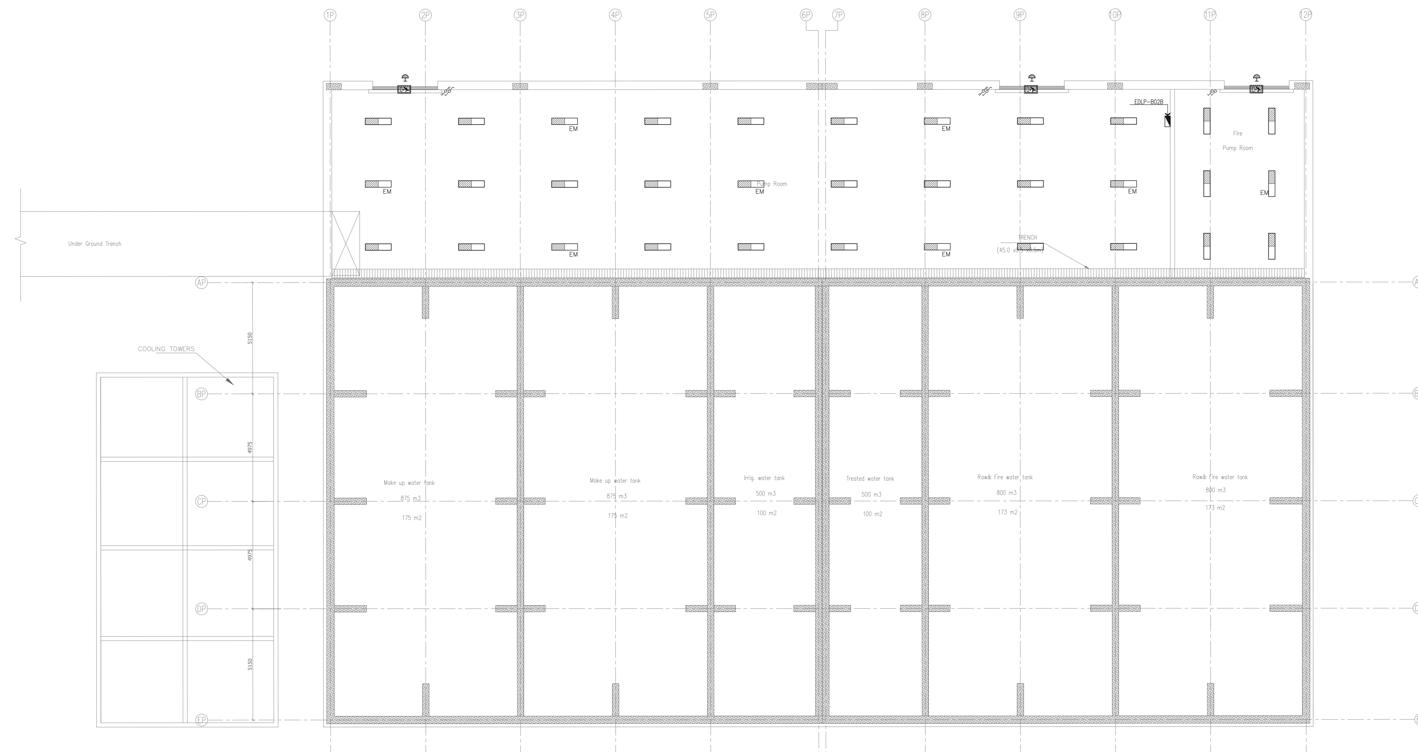
① GROUND FLOOR LIGHTING LAYOUT SCALE: 1:100
